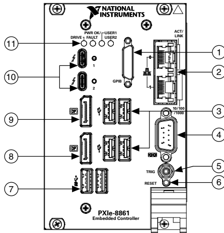
Figure 3. PXIe-8861 Front Panel Layout
