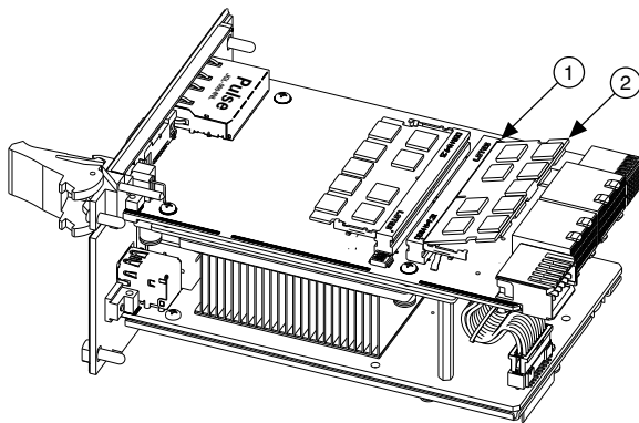
Figure 5. Installing a SO-DIMM in a PXIe-8861 Controller
