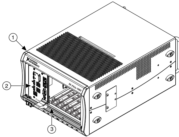
Figure 2. PXIe-8861 Installed in a PXI Express Chassis
