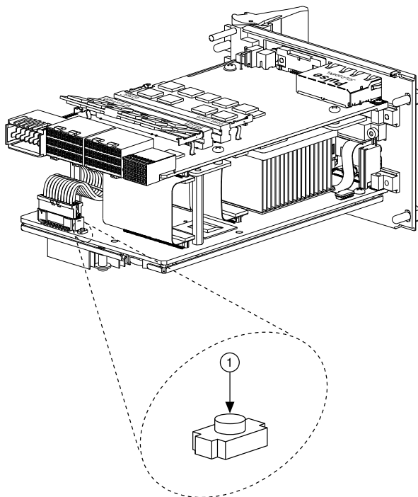
Figure 6. Clearing the CMOS Contents
