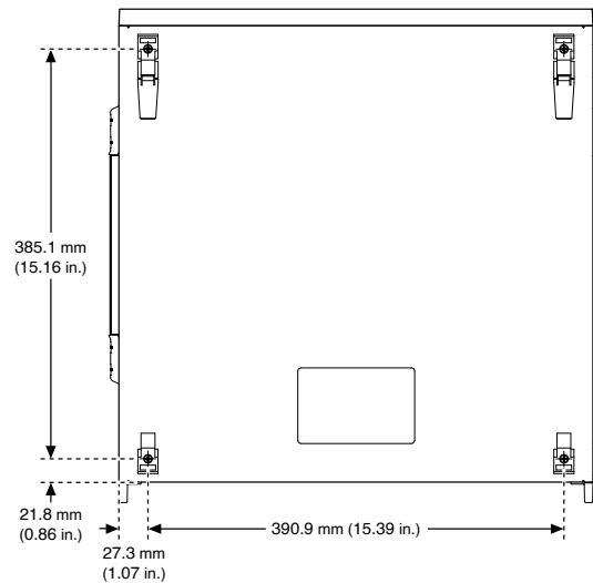
Figure 1. PXIe-1084 Chassis Dimensions (Bottom)
