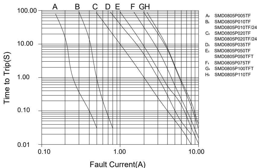
SMD0805 Series TTT Vs Fault current chart
