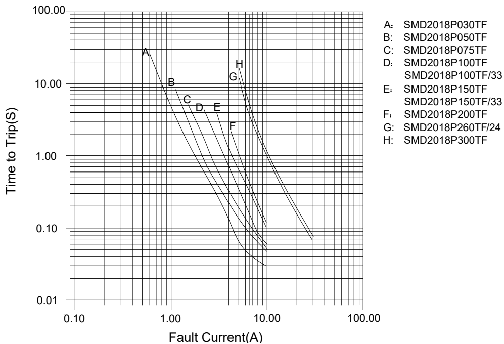
SMD2018 Series TTT Vs Fault current chart
