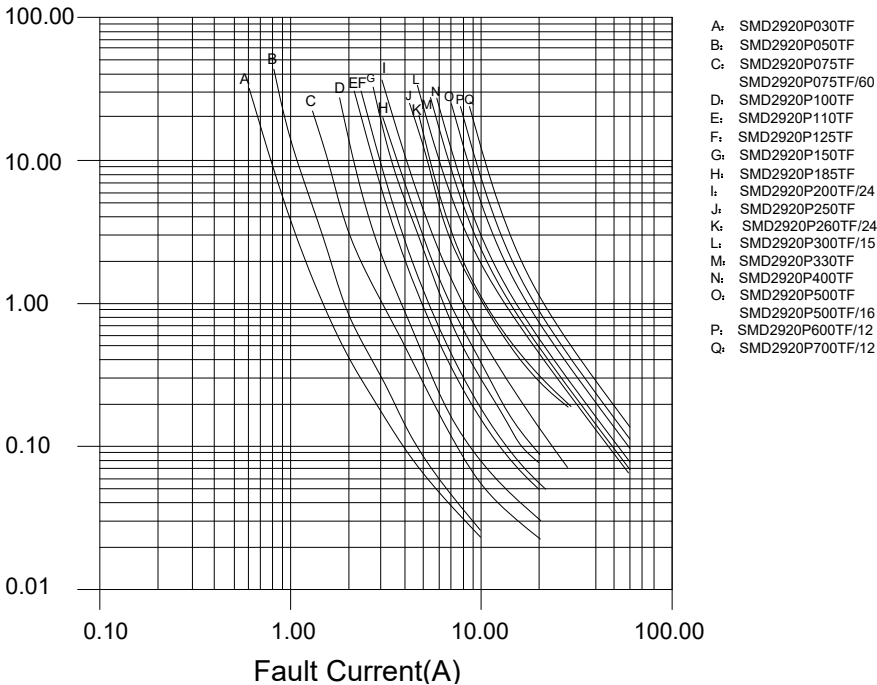
SMD2920 Series TTT Vs Fault current chart
